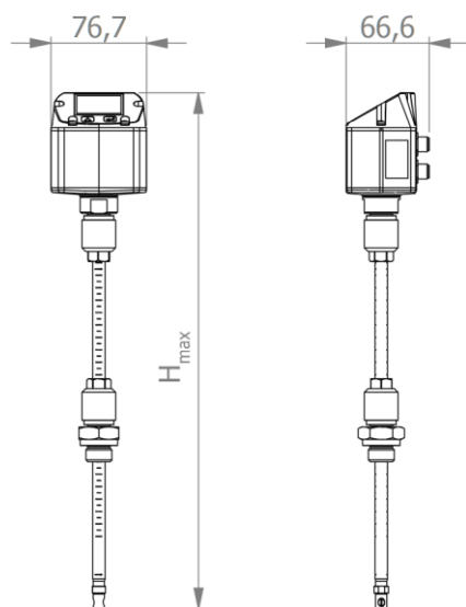
Figure 33: Dimensions
