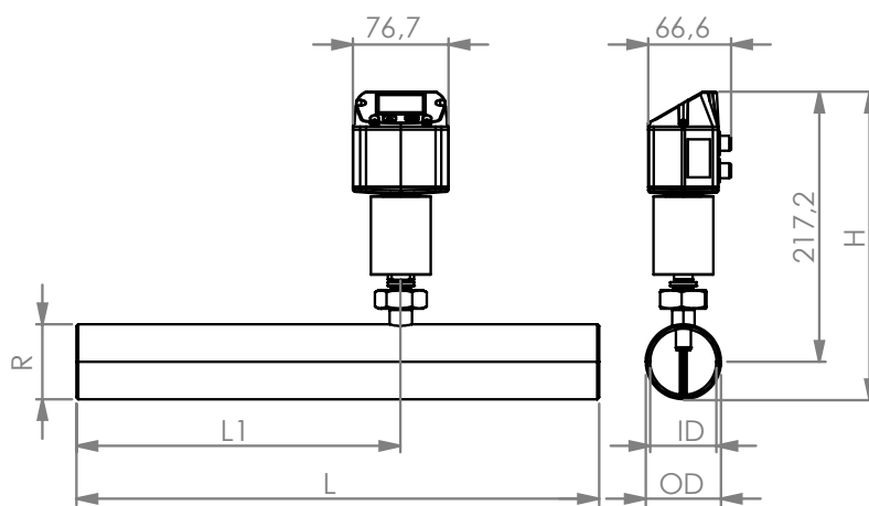
Figure 31: Dimensions
