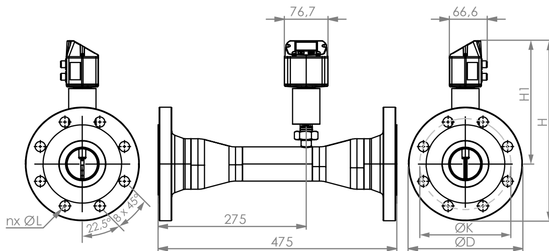
Figure 33: Dimensions
