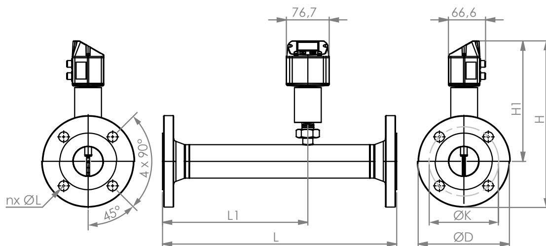
Figure 32: Dimensions
